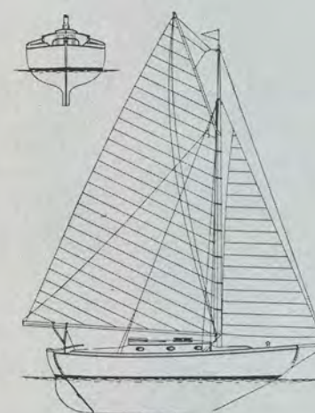
NOORSE JOL
