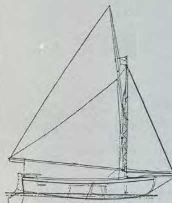
SCHELDE JOL
